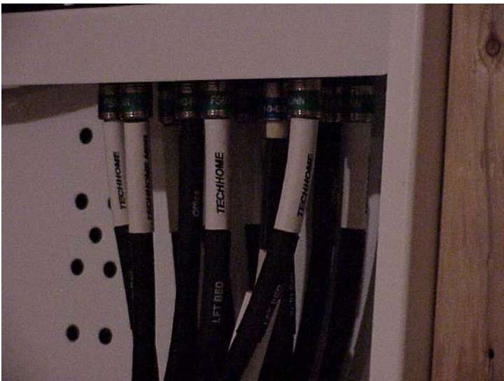
RG 6 Quad Shield
